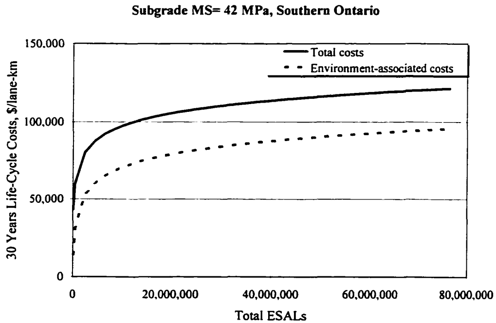
Figure 3.21. Environment and Traffic Costs vs Total ESALs, Southern Ontario
