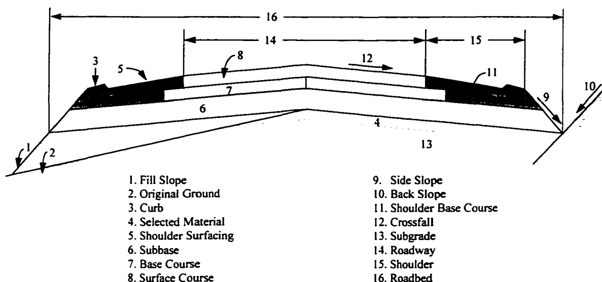
Figure 3.1. Typical Flexible Pavement Structure (Modified from TAC, 1997)
