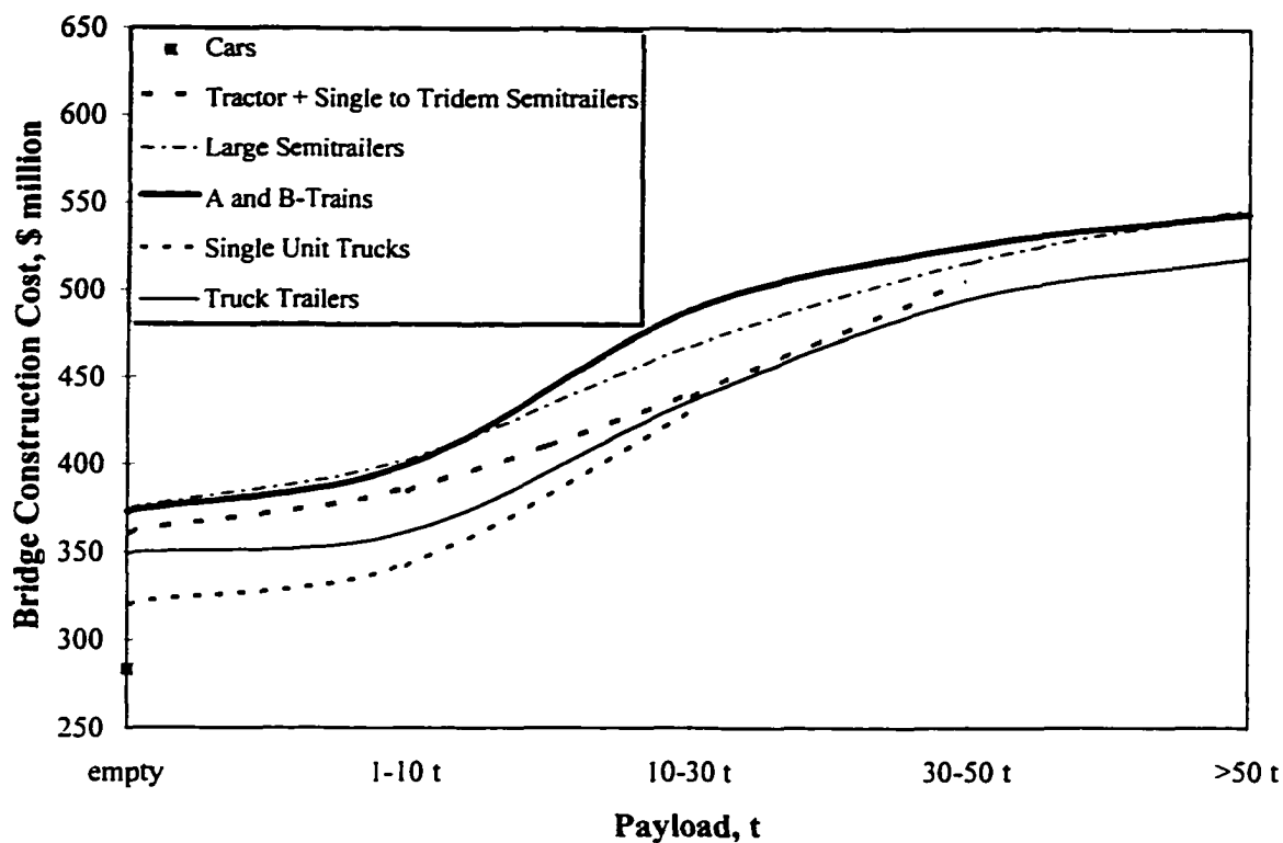
Figure 6.11. Annualized Bridge Construction Costs for Different Loads
