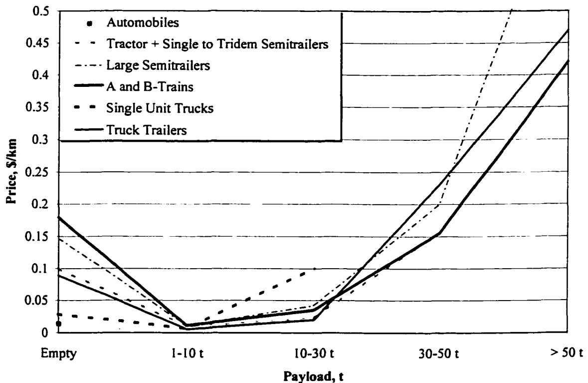
Figure 8.2. Pavement and Bridge Price vs Payload for Different Truck Types
